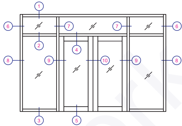
TYPICAL ELEVATION
