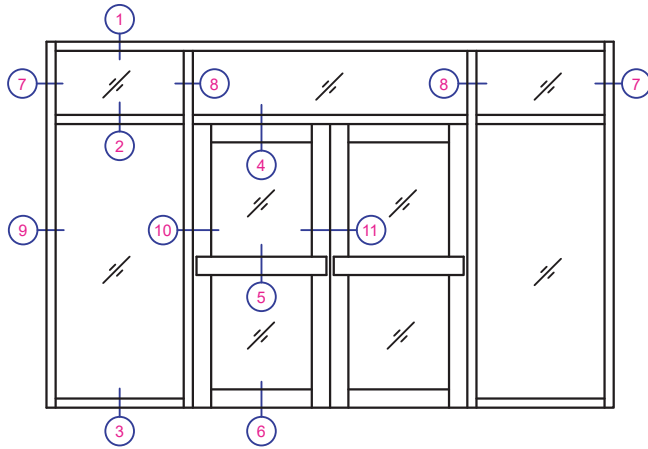
TYPICAL ELEVATION
