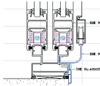
2-track system
