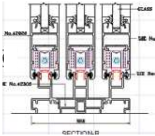
3-track system
